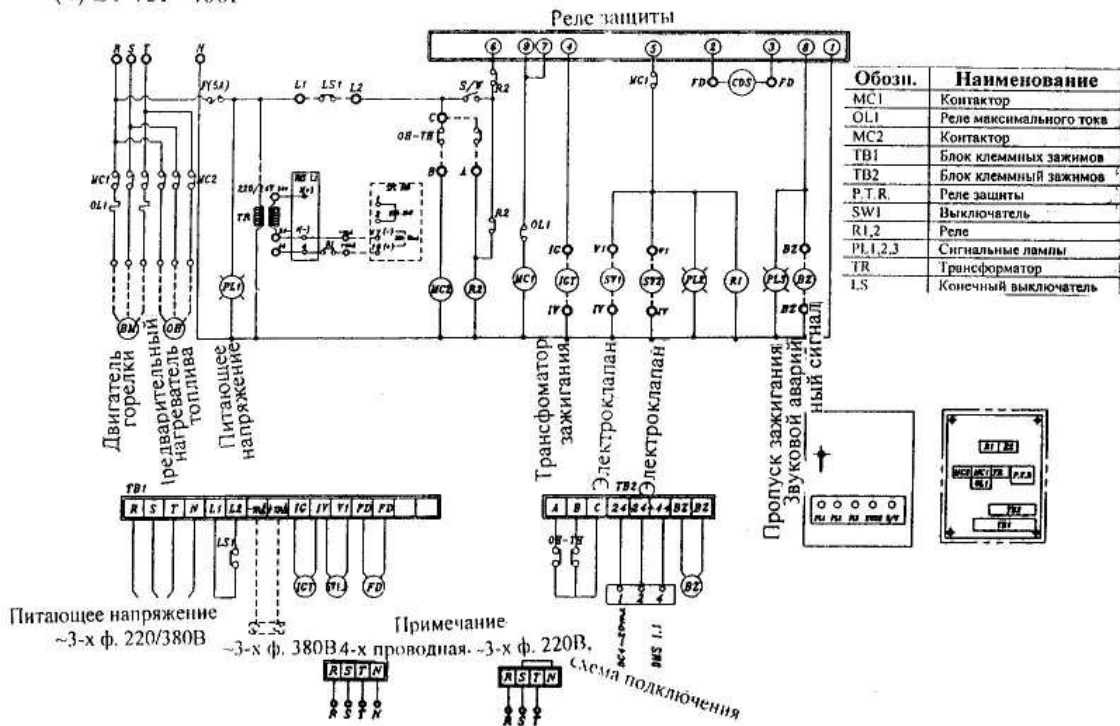
(4) LT-75P~400P
